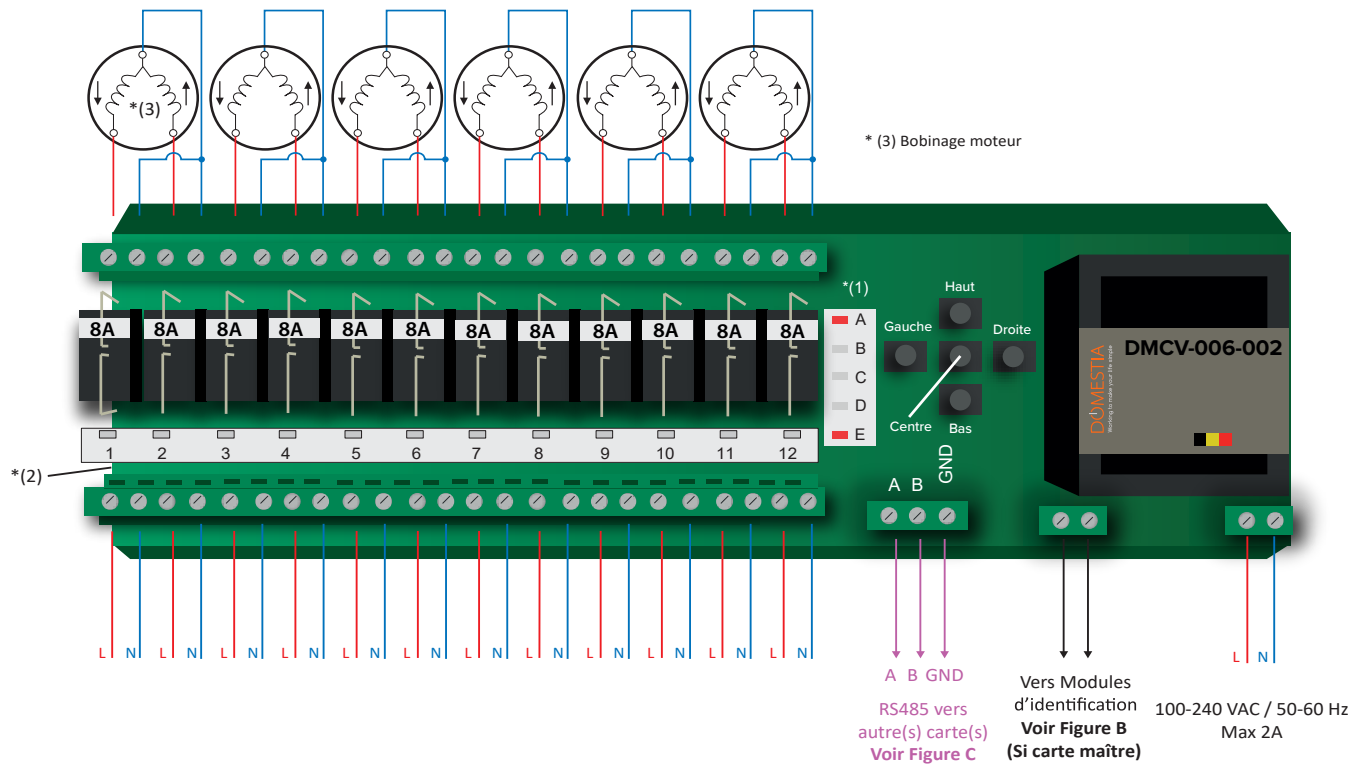
FIGURE A - Carte de base DMCV-006-002 (exemple de raccordement)
